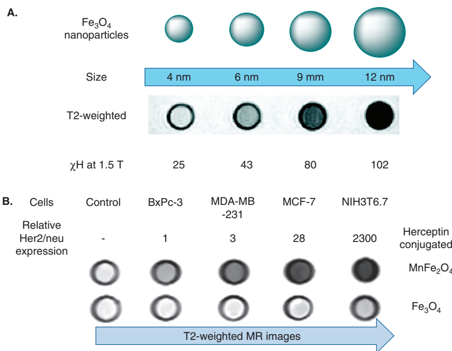
Figure 3. A. Illustration of size-dependent T2-weighted images and mass magnetization of iron oxide nanoparticles at 1.5 T. B. Magnetic resonance contrast T2-weighted images with different HER2/neu expression levels.
